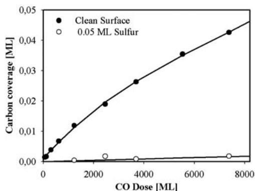
Fig. 7 The experimentally determined carbon coverage on a Ni(14 13 13) single crystal as a function of the CO exposure at 500 K. Results are shown for both the clean surface and for a surface that has been pre-exposed to 0.05 ML of sulfur which is known to preferentially block the steps. The surface is incapable of dissociating the CO when the steps are blocked. Adapted from ref. 47.
